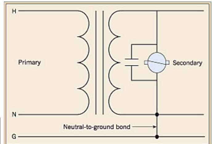
Fig. 3. An "ABC"-style plug-in power conditioner incorporates a surge diverter, isolation transformer, and power line noise filter.
