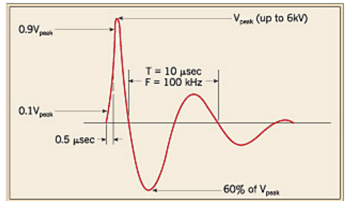
Fig. 2. Graph of a typical type of “ringing” transient often found at the end of a long branch circuit, where most computer equipment is installed.
