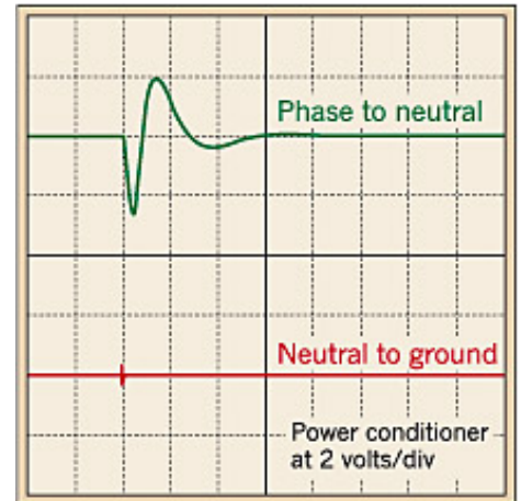
Fig. 5. A 1,000V impulse injected between phase and neutral at the input to an “ABC”-style plug-in power conditioner. Note that the phase-to-neutral impulse (normal mode) is attenuated to less than 10V while less than 0.5V appears between neutral and ground at the output.
